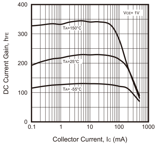
Fig.1 - h_{FE} vs. I_C (ABC817-16W-HF)
