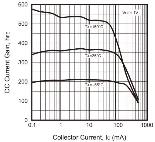
Fig.2 - h_{FE} vs. I_C (ABC817-25W-HF)
