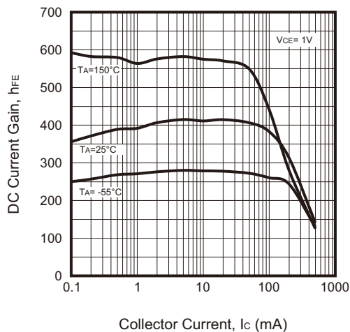
Fig.3 - h_{FE} vs. I_C (ABC817-40W-HF)
